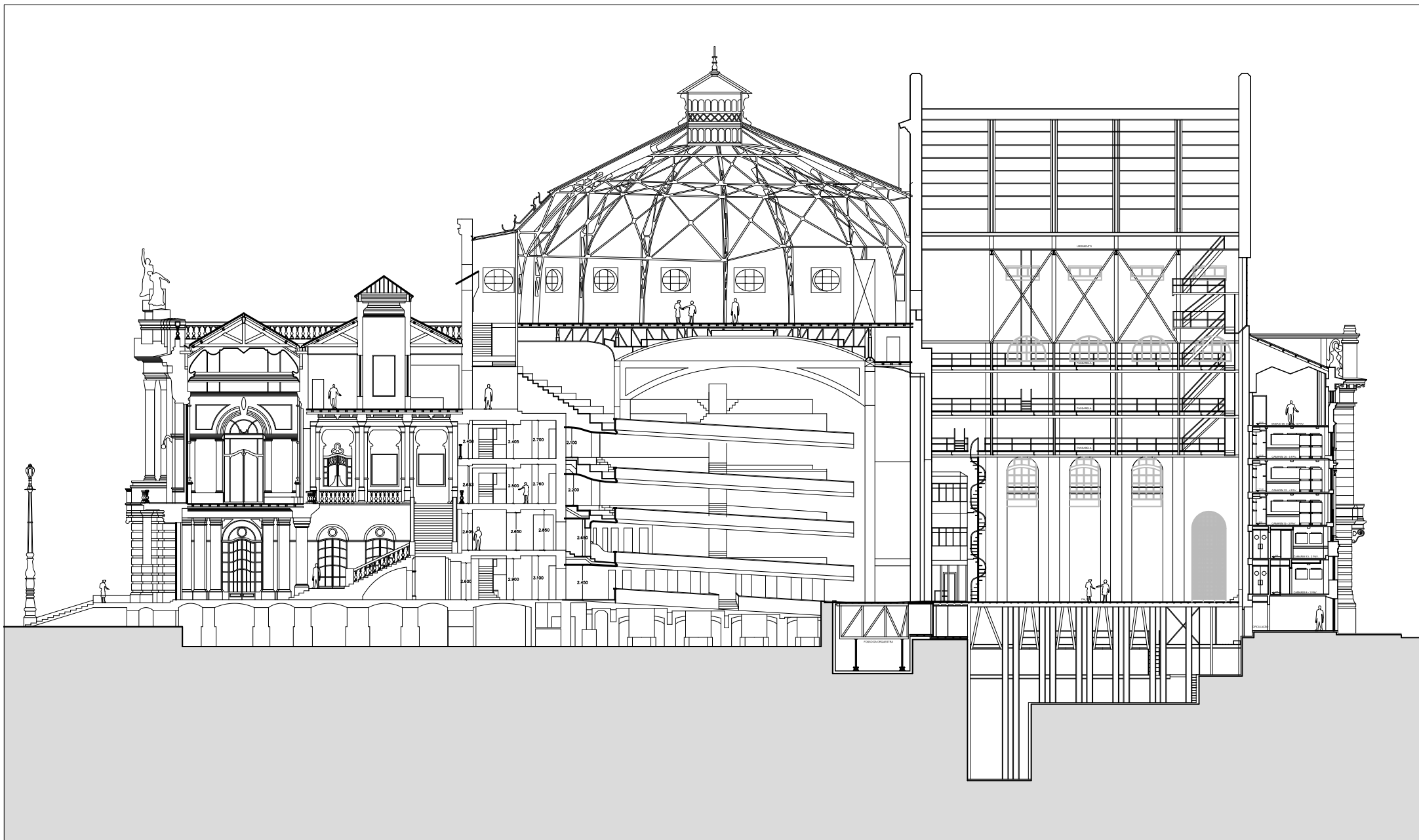
TMSP - THEATRO MUNICIPAL DE SÃO PAULO CORTE AA'
